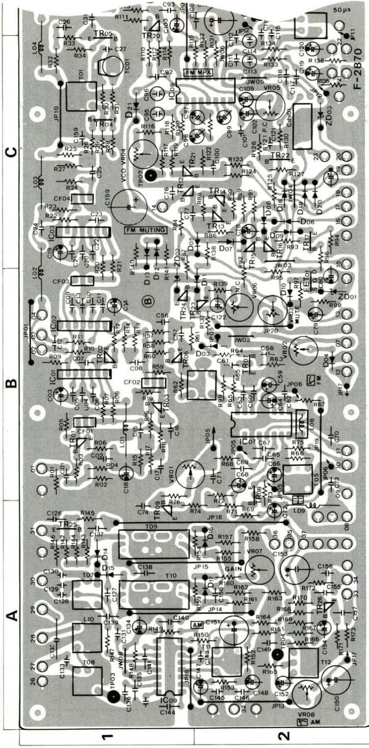
3-1. F-2870 Tuner Circuit Board (Stock No. 7522251)
